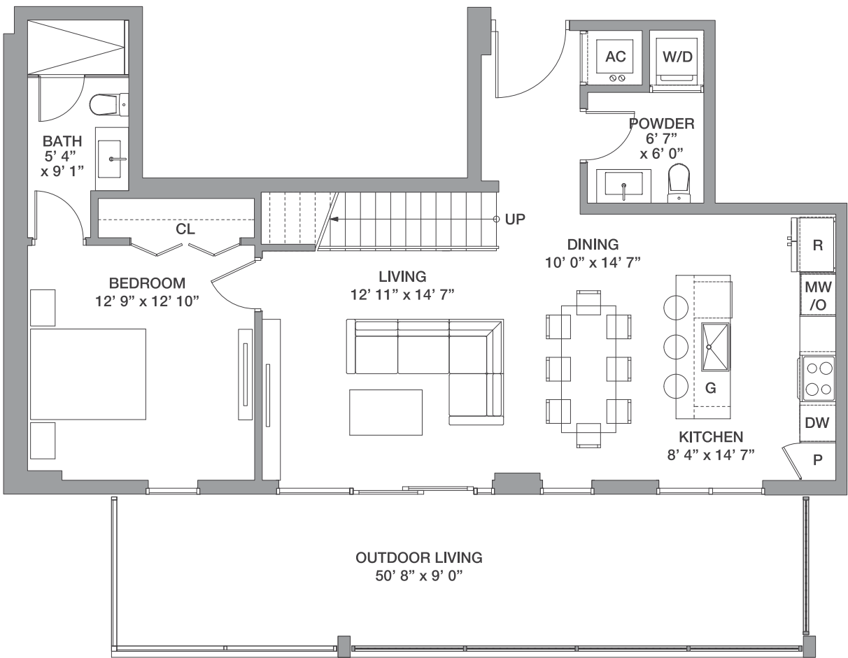
LOWER LEVEL
