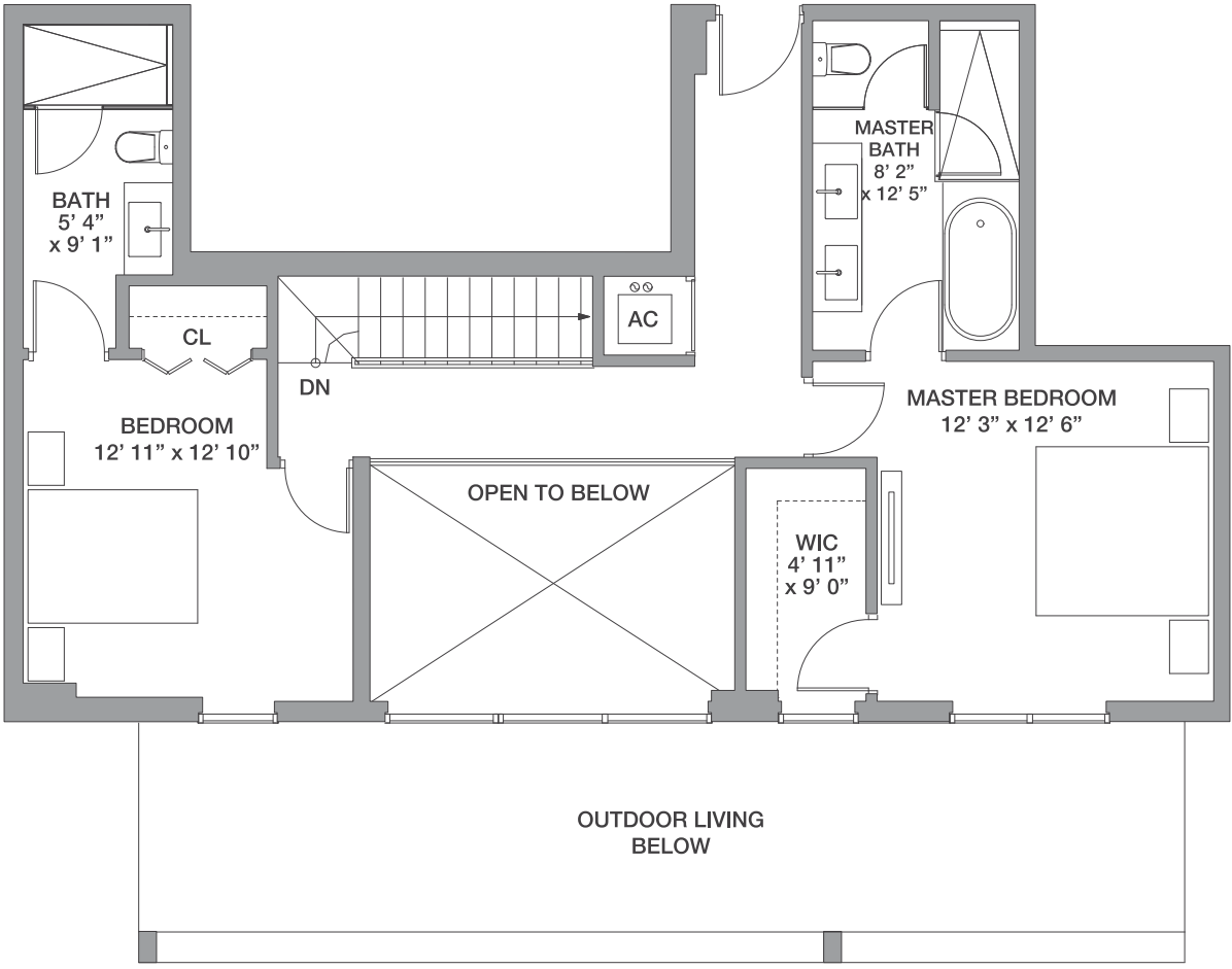
UPPER LEVEL
