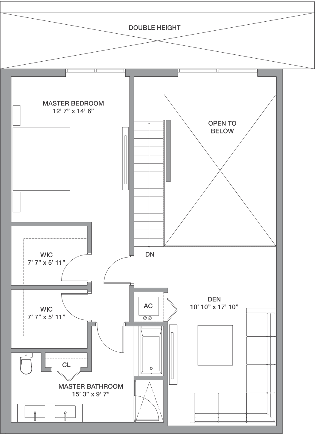
UPPER LEVEL
